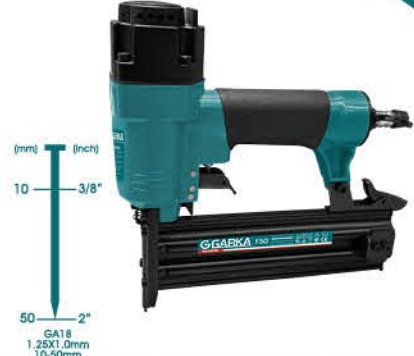
Brad nailer
